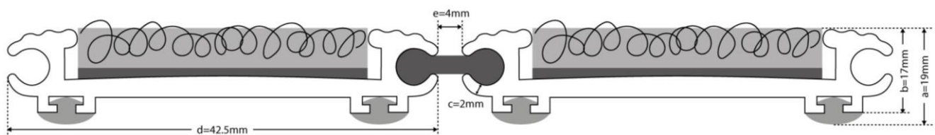
Figure 1: Cross section of ALTAC Aluminium Mat System
